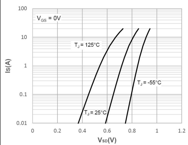
Figure 6. Body Diode Characteristics
