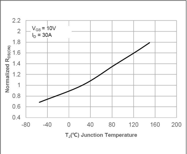
Figure 8. Normalized on Resistance vs Junction
