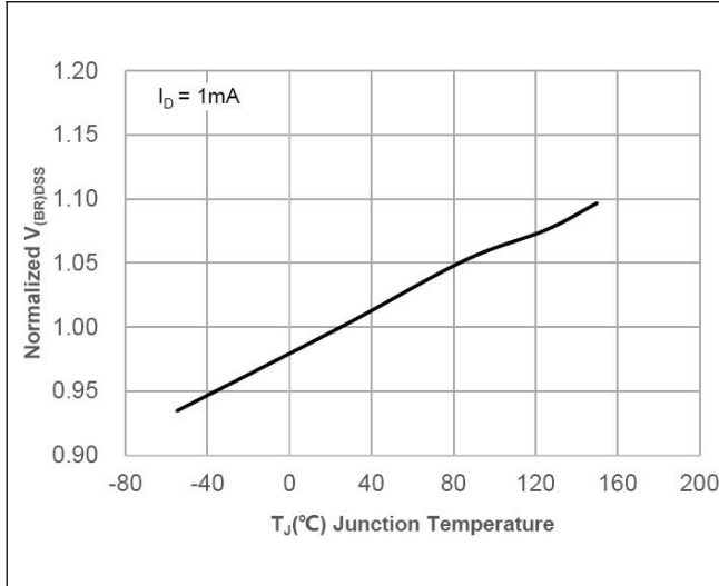
Figure 7. Normalized Breakdown voltage vs Junction
